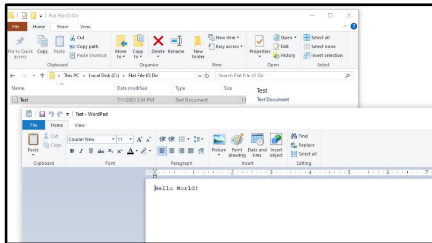
Figure 10.4: Output
