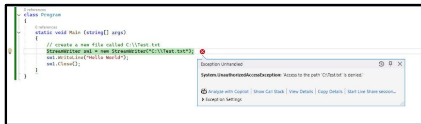
Figure 10.1: UnauthorizedAccessException
